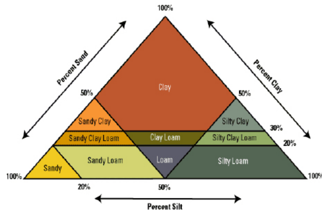
Figure 1. USDA Soil Classification System
